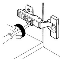
Height adjustment
