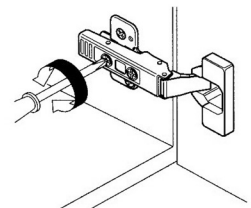
Depth adjustment
